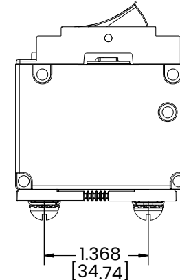
BACK CONNECT SCREW TERMINAL WITH RETAINER-ALTERNATIVE SPACING
