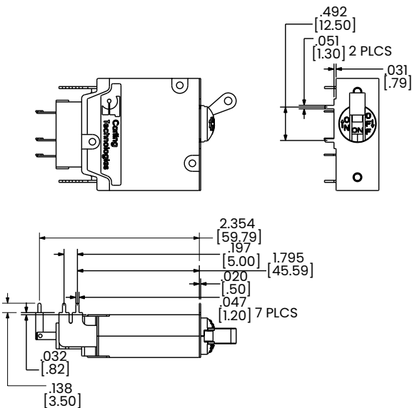
PRINTED CIRCUIT BOARD MOUNTING TERMINAL CODE R
