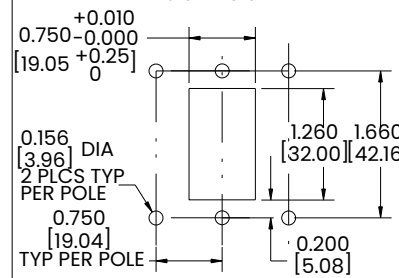
PANEL CUT-OUT DETAIL
